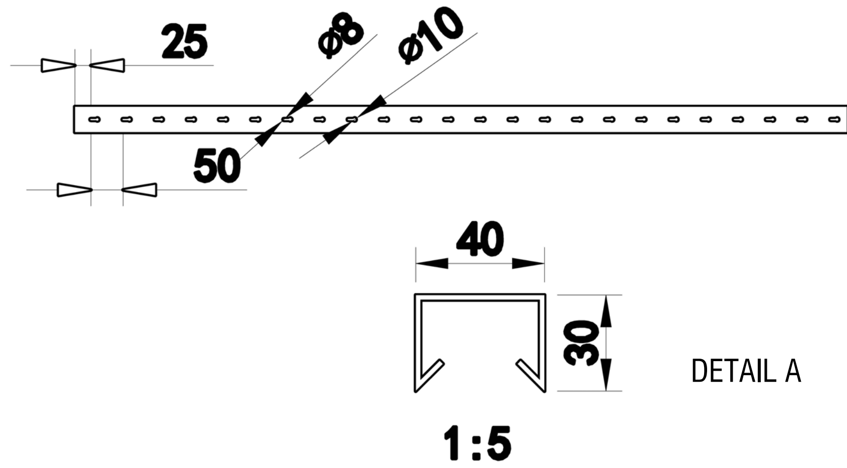
1 PLAN VIEW & HARDWARE DETAILS
