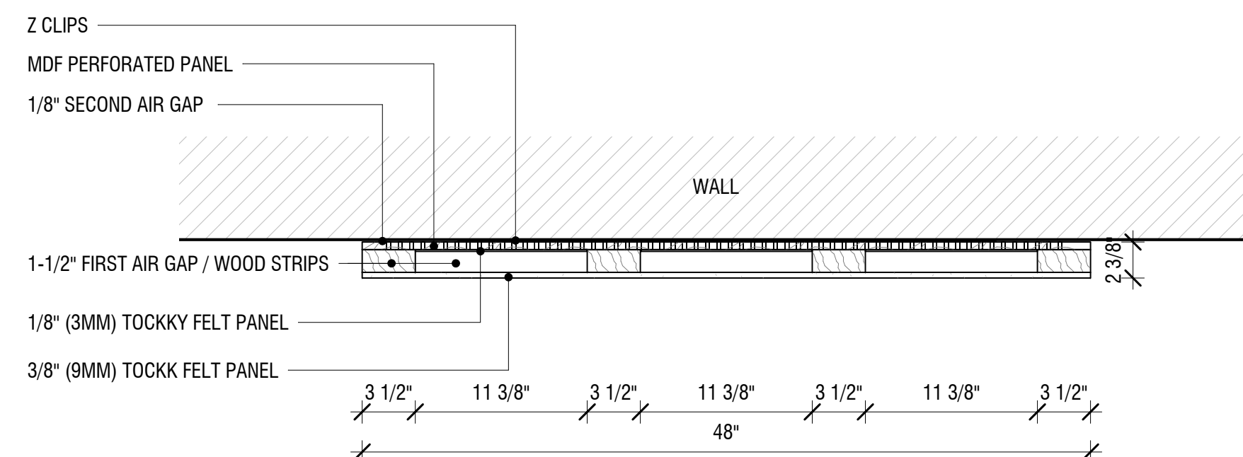
3/8" TOCKKY PANEL OMEGA DUAL PANEL W/BUILT-IN AIR GAP - 4'x9' - 1ST STYLE - PLAN VIEW ① 1 1/2" = 1'-0"
