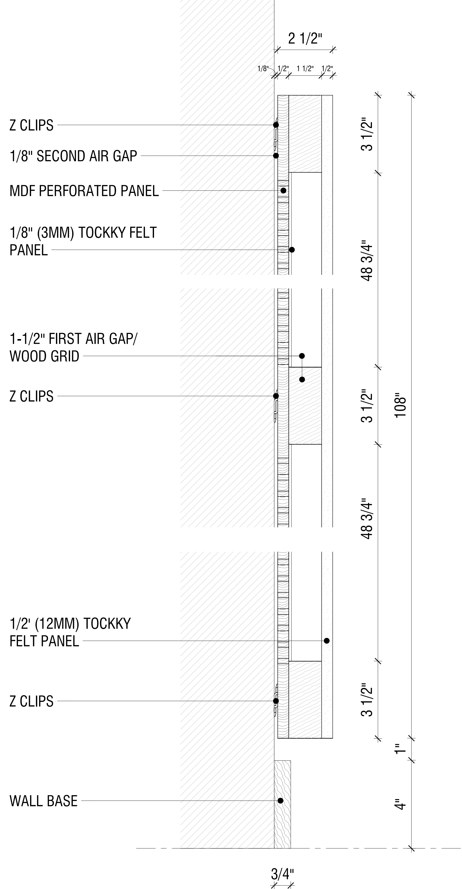
1/2" TOCKKY PANEL OMEGA DUAL PANEL W/BUILT-IN AIR GAP - 4'x9' - 1ST STYLE - SECTIONAL DETAIL 6" = 1'-0"
