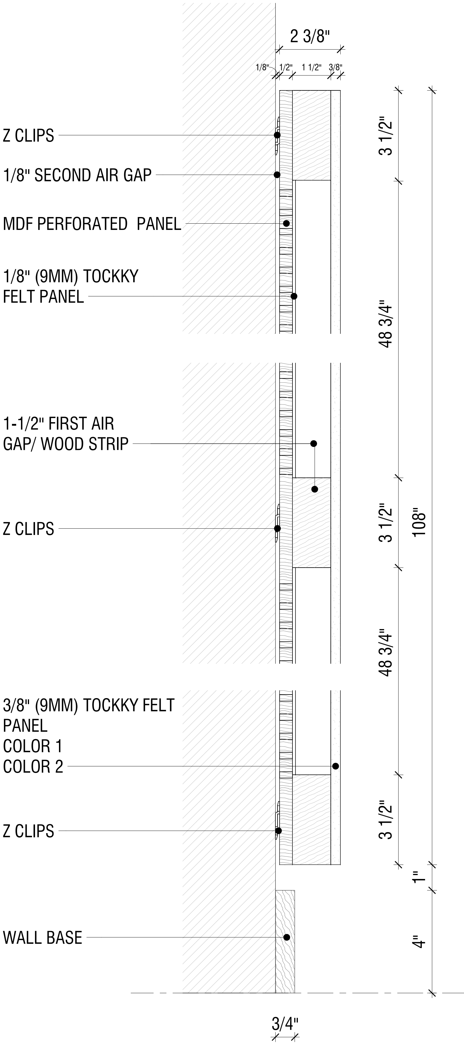
3/8" TOCKKY PANEL OMEGA DUAL PANEL W/BUILT-IN AIR GAP - 4'x9' - 2ND STYLE - SECTIONAL DETAIL 6" = 1'-0"
