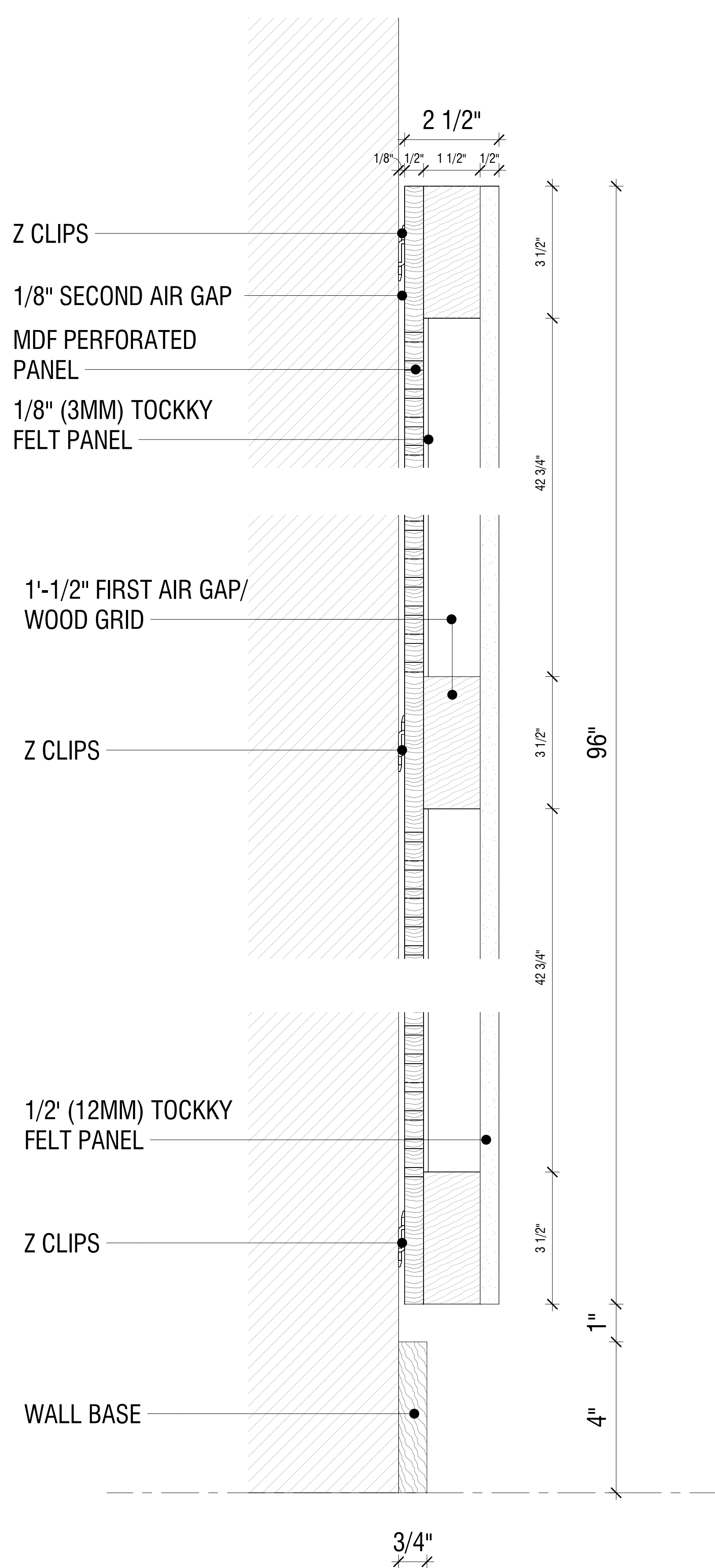
1/2" TOCKKY PANEL OMEGA DUAL PANEL W/BUILT-IN AIR GAP - 4'x8' - 1ST STYLE - SECTIONAL DETAIL ④ 6" = 1'-0"
