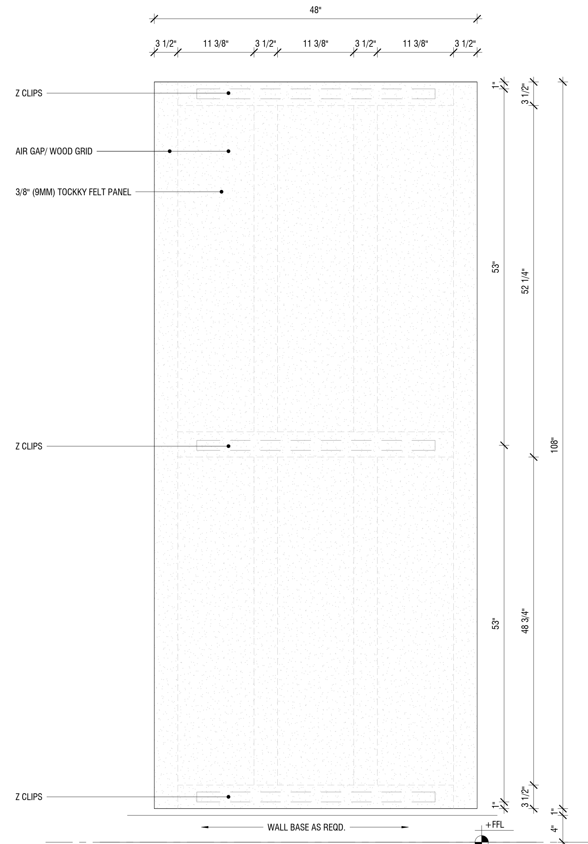
3/8" TOCKKY PANEL OMEGA DUAL PANEL W/BUILT-IN AIR GAP - 4'x9' - 1ST STYLE - ELEVATION ② 1 1/2" = 1'-0"
