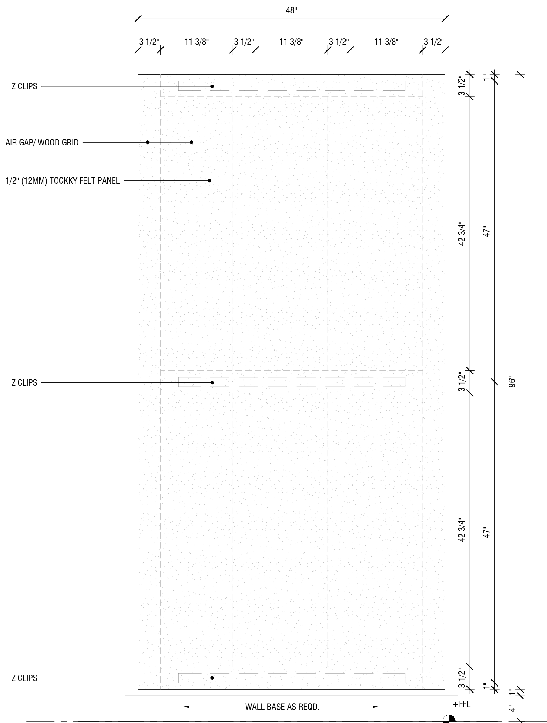
1/2" TOCKKY PANEL OMEGA DUAL PANEL W/BUILT-IN AIR GAP - 4'x8' - 1ST STYLE - ELEVATION ② 1 1/2" = 1'-0"
