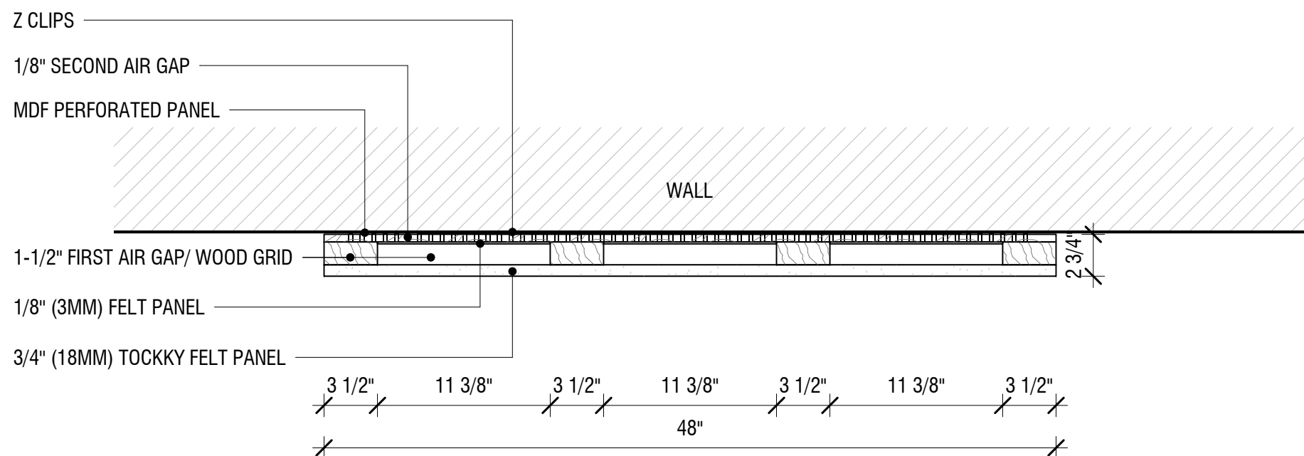
3/4" TOCKKY PANEL OMEGA DUAL PANEL W/BUILT-IN AIR GAP - 4'x9' - 1ST STYLE STYLE - PLAN VIEW 1 1/2" = 1'-0"
