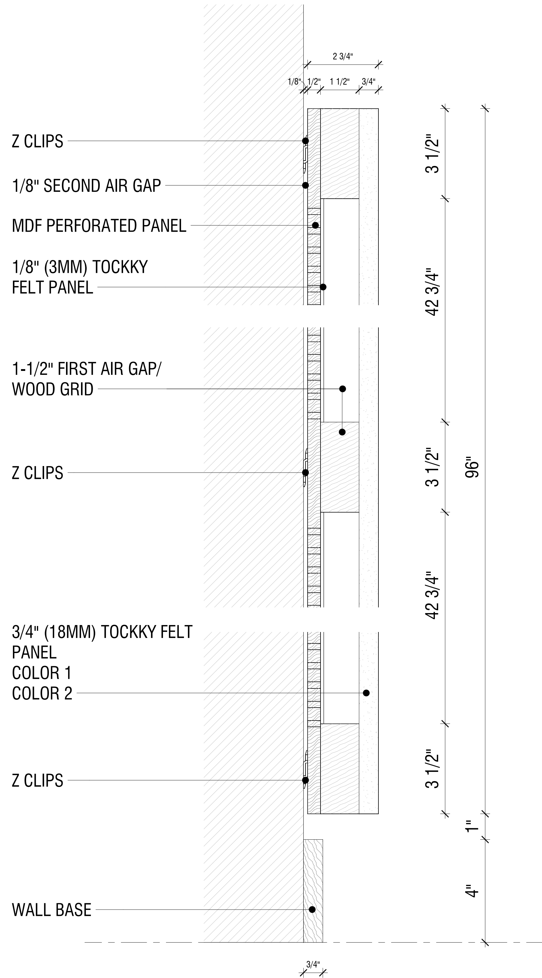
3/4" TOCKKY PANEL OMEGA DUAL PANEL W/BUILT-IN AIR GAP - 4'x8' - 2ND STYLE STYLE - SECTIONAL DETAIL ④ 6" = 1'-0"
