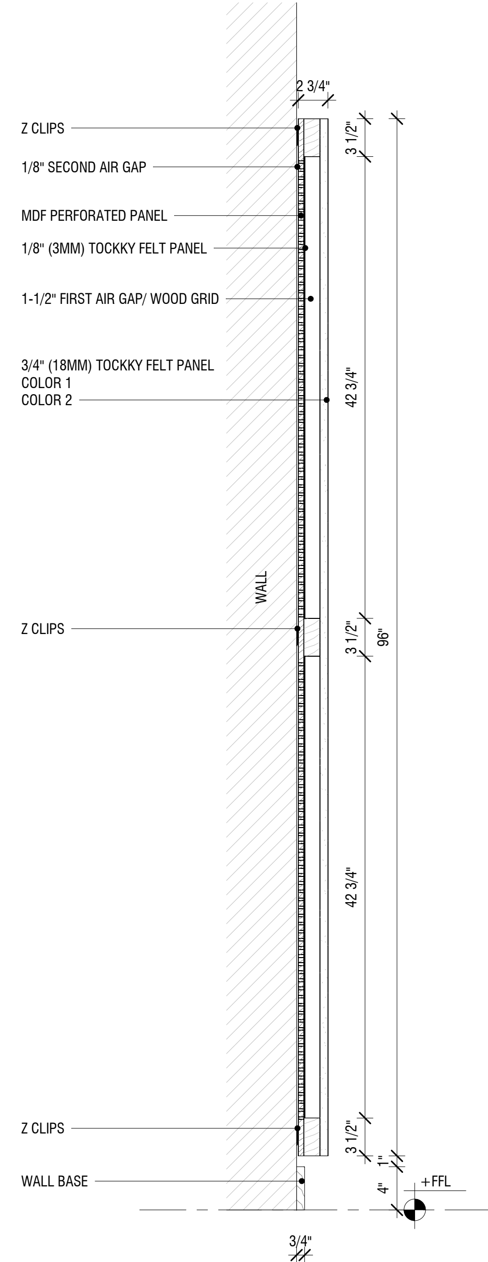
3/4" TOCKKY PANEL OMEGA DUAL PANEL W/BUILT-IN AIR GAP - 4'x8' - 2ND STYLE STYLE - TYP. SECTION ③ 1 1/2" = 1'-0"
