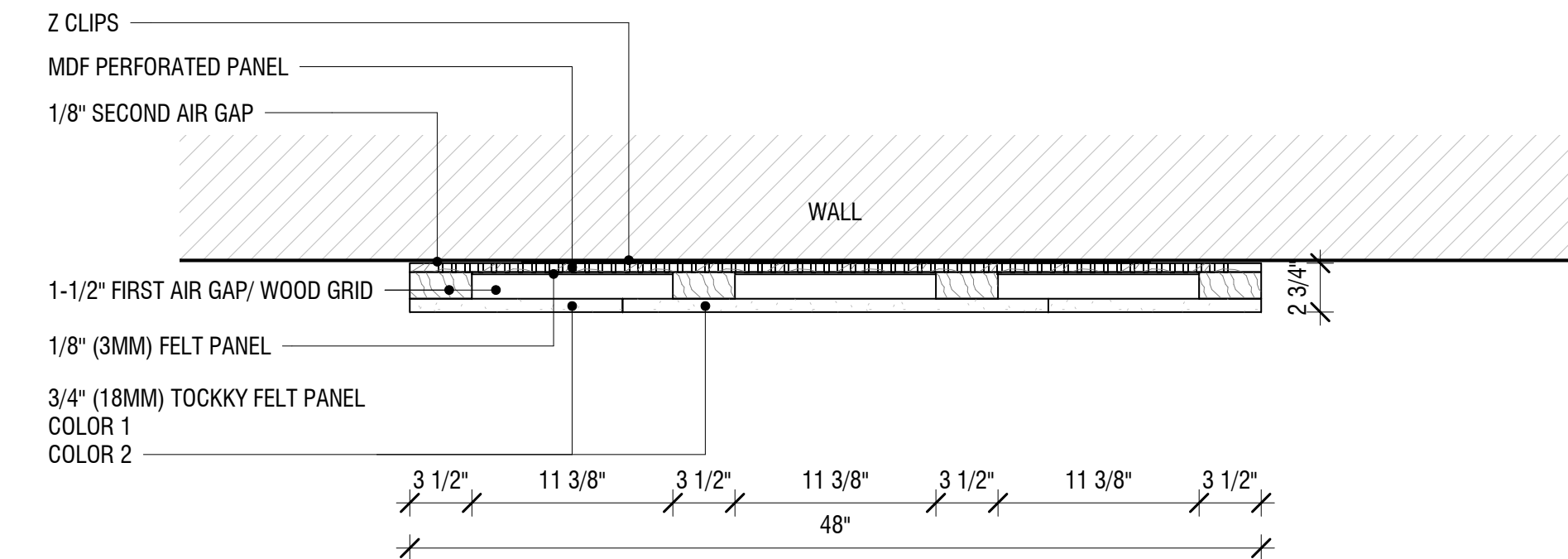
3/4" TOCKKY PANEL OMEGA DUAL PANEL W/BUILT-IN AIR GAP - 4'x8' - 2ND STYLE STYLE - PLAN VIEW ① 1 1/2" = 1'-0"
