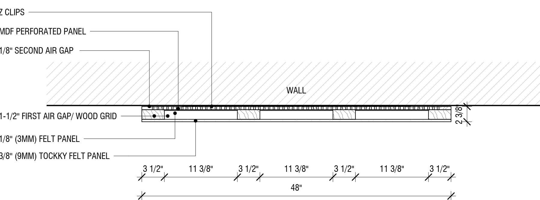
3/8" TOCKKY PANEL OMEGA DUAL PANEL W/BUILT-IN AIR GAP - 4'x8' - 1ST STYLE - PLAN VIEW 1 1/2" = 1'-0"
