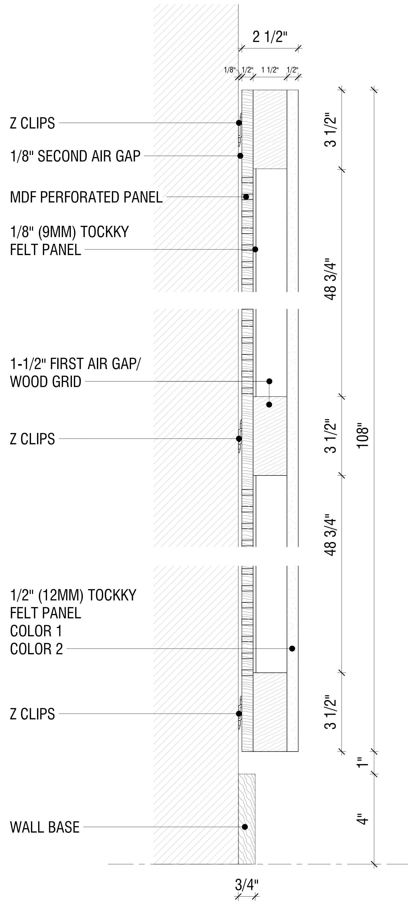
1/2" TOCKKY PANEL OMEGA DUAL PANEL W/BUILT-IN AIR GAP - 4'x9' - 2ND STYLE - SECTIONAL DETAIL 6" = 1'-0"
