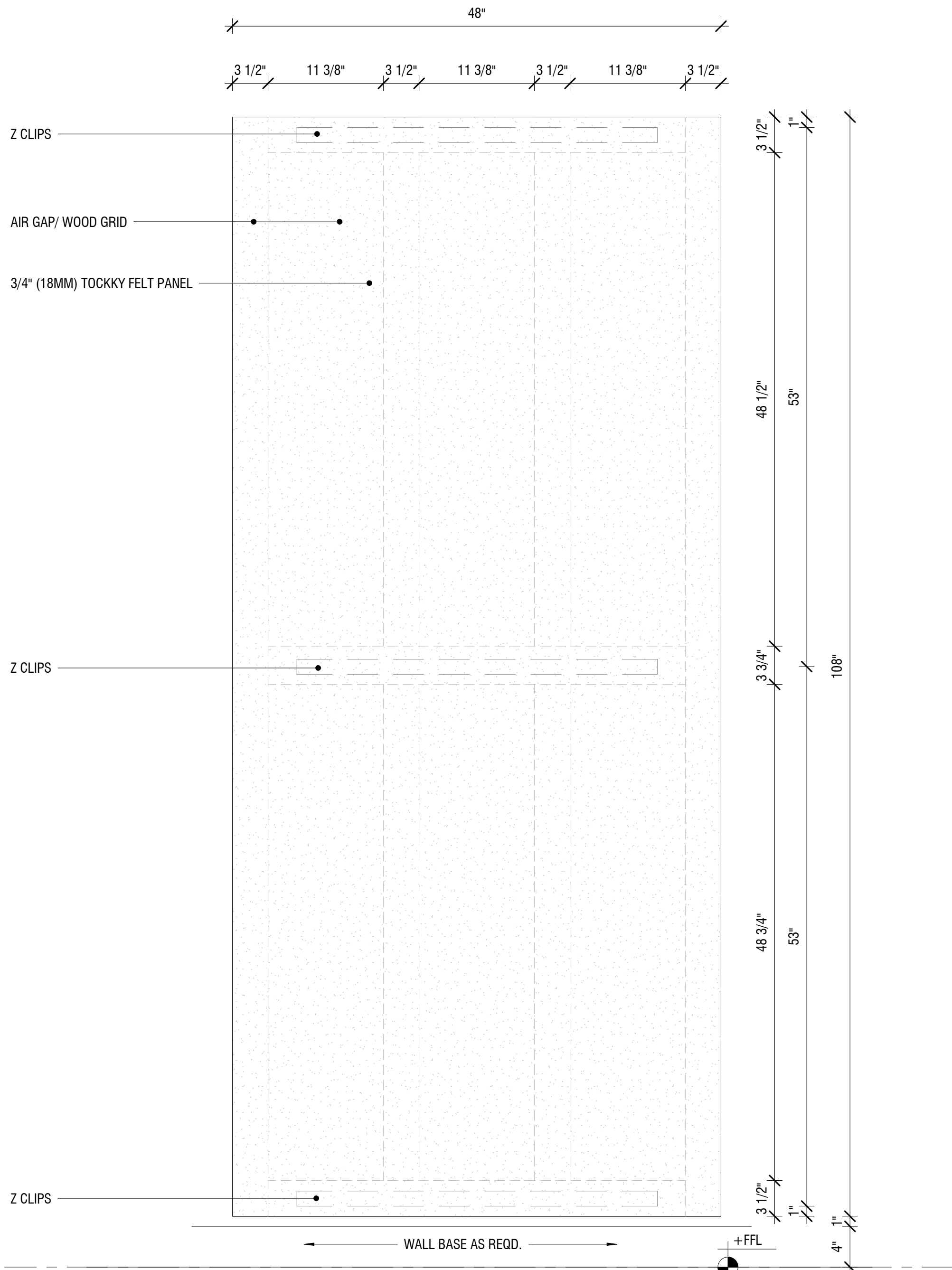
3/4" TOCKKY PANEL OMEGA DUAL PANEL W/BUILT-IN AIR GAP - 4'x9' - 1ST STYLE STYLE - ELEVATION 1 1/2" = 1'-0"
