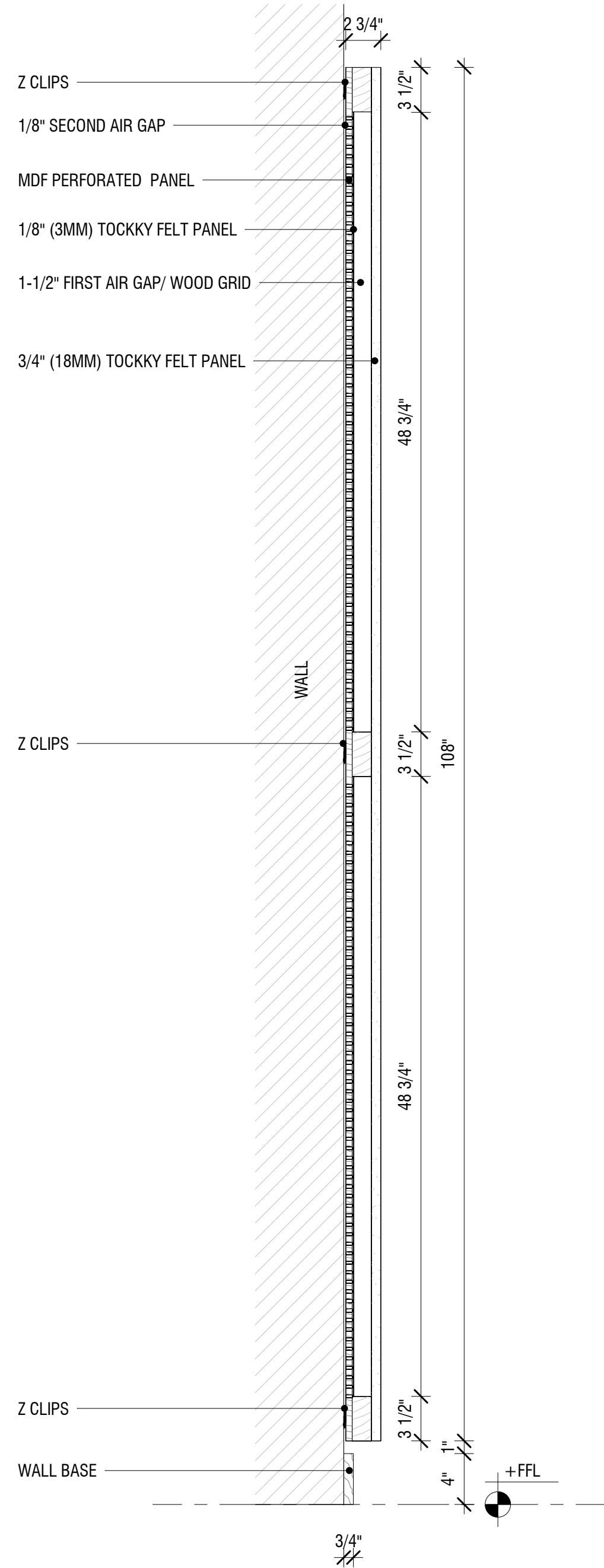
3/4" TOCKKY PANEL OMEGA DUAL PANEL W/BUILT-IN AIR GAP - 4'x9' - 1ST STYLE STYLE - TYP. SECTION 1 1/2" = 1'-0"
