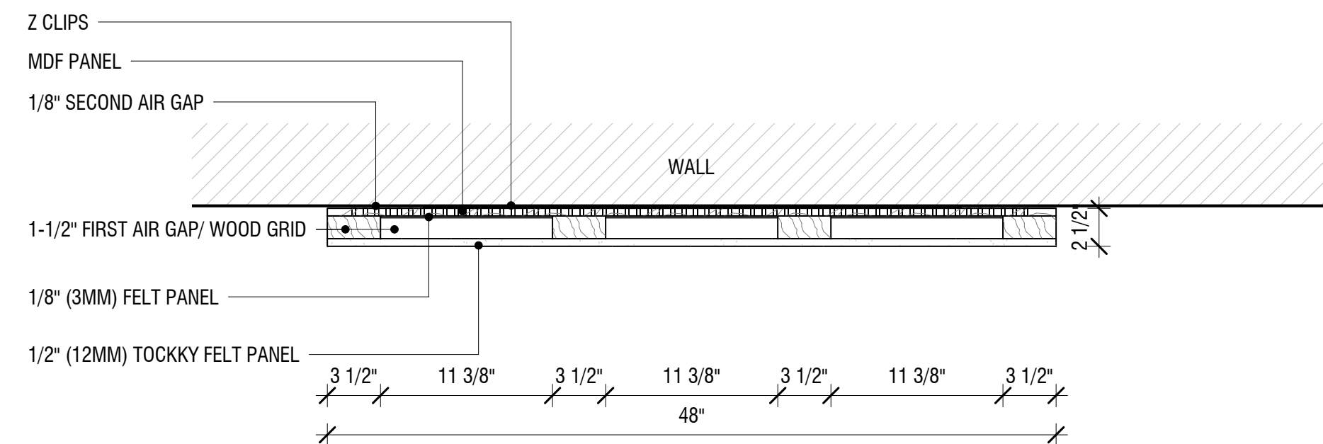
1/2" TOCKKY PANEL OMEGA DUAL PANEL W/BUILT-IN AIR GAP - 4'x9' - 1ST STYLE - PLAN VIEW 1 1/2" = 1'-0"
