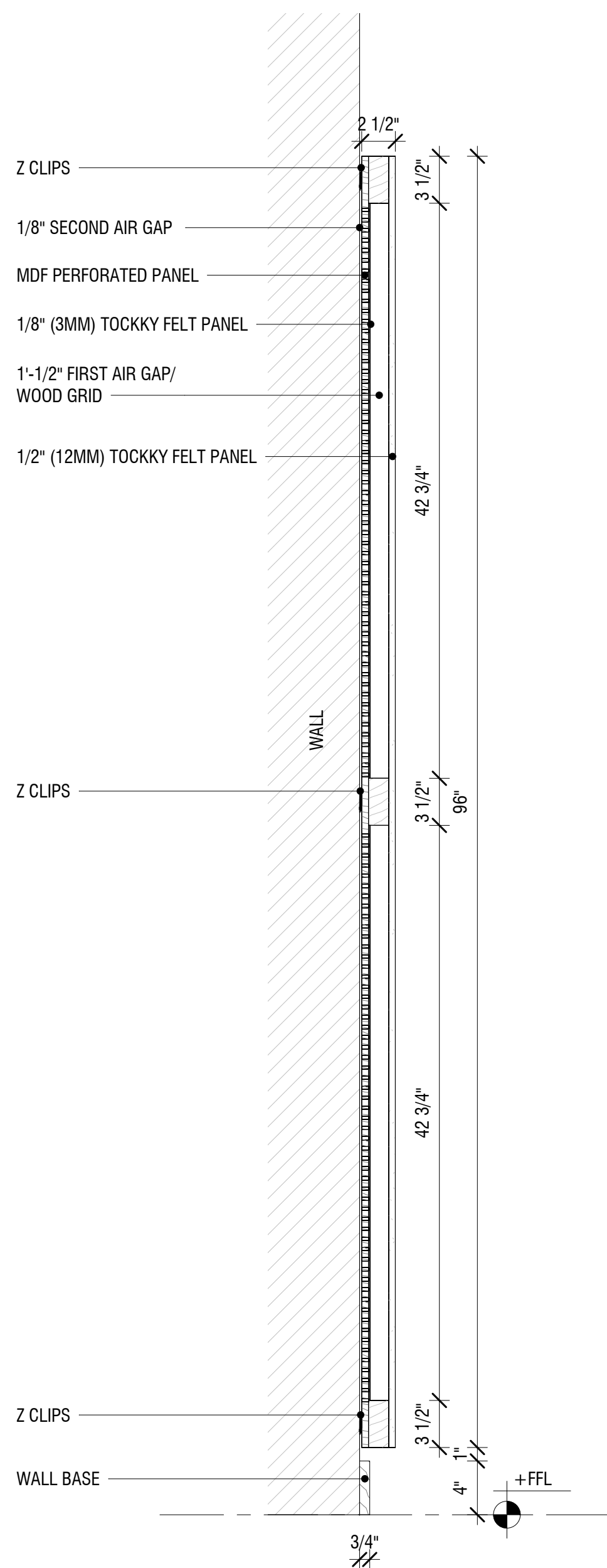
1/2" TOCKKY PANEL OMEGA DUAL PANEL W/BUILT-IN AIR GAP - 4'x8' - 1ST STYLE - TYP. SECTION ③ 1 1/2" = 1'-0"
