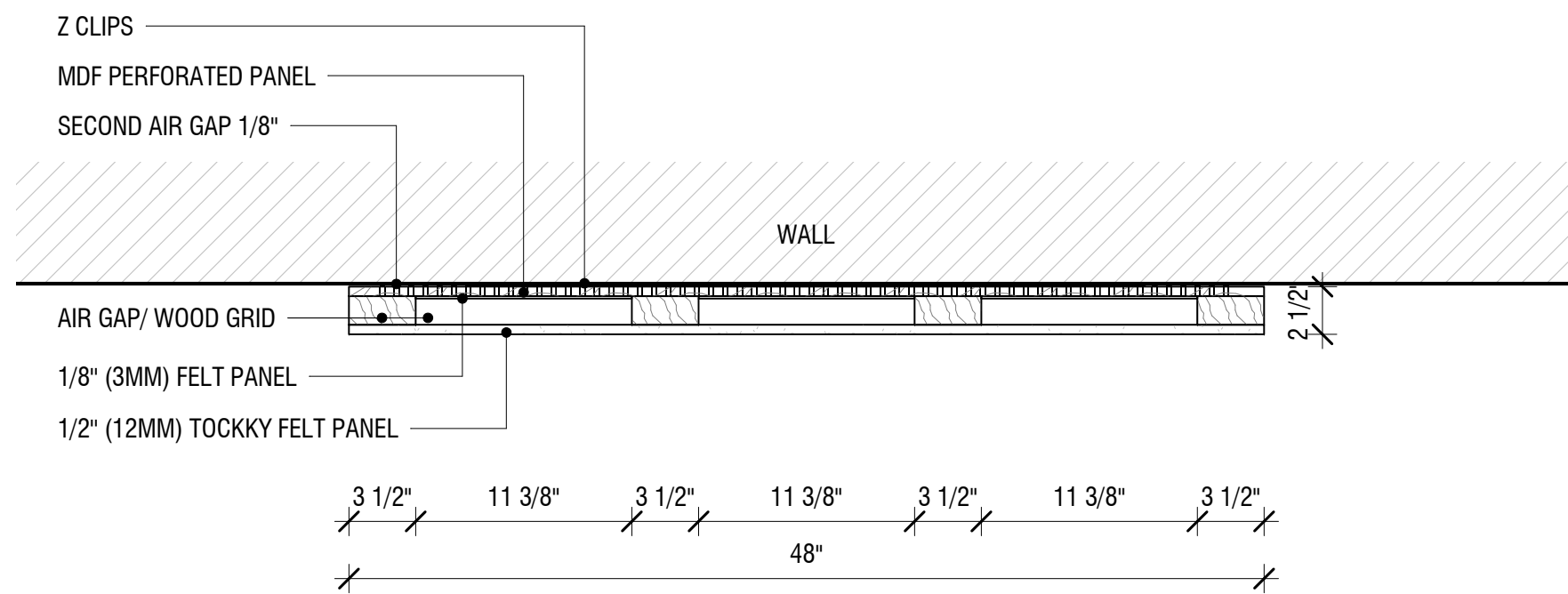
1/2" TOCKKY PANEL OMEGA DUAL PANEL W/BUILT-IN AIR GAP - 4'x8' - 1ST STYLE - PLAN VIEW ① 1 1/2" = 1'-0"
