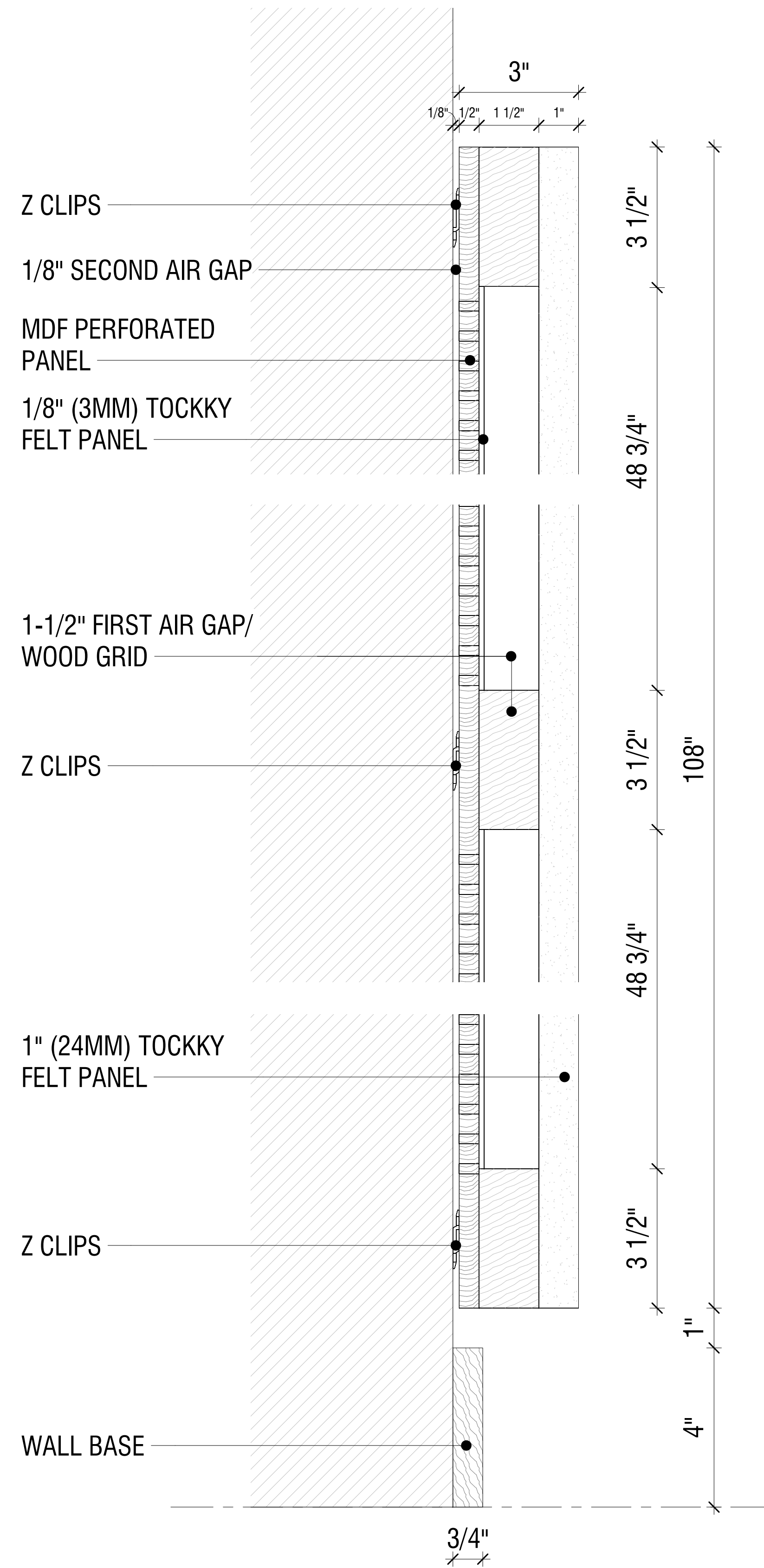
1" TOCKKY PANEL OMEGA DUAL PANEL W/BUILT-IN AIR GAP - 4'x9' - 1ST STYLE - SECTIONAL DETAIL 6" = 1'-0"
