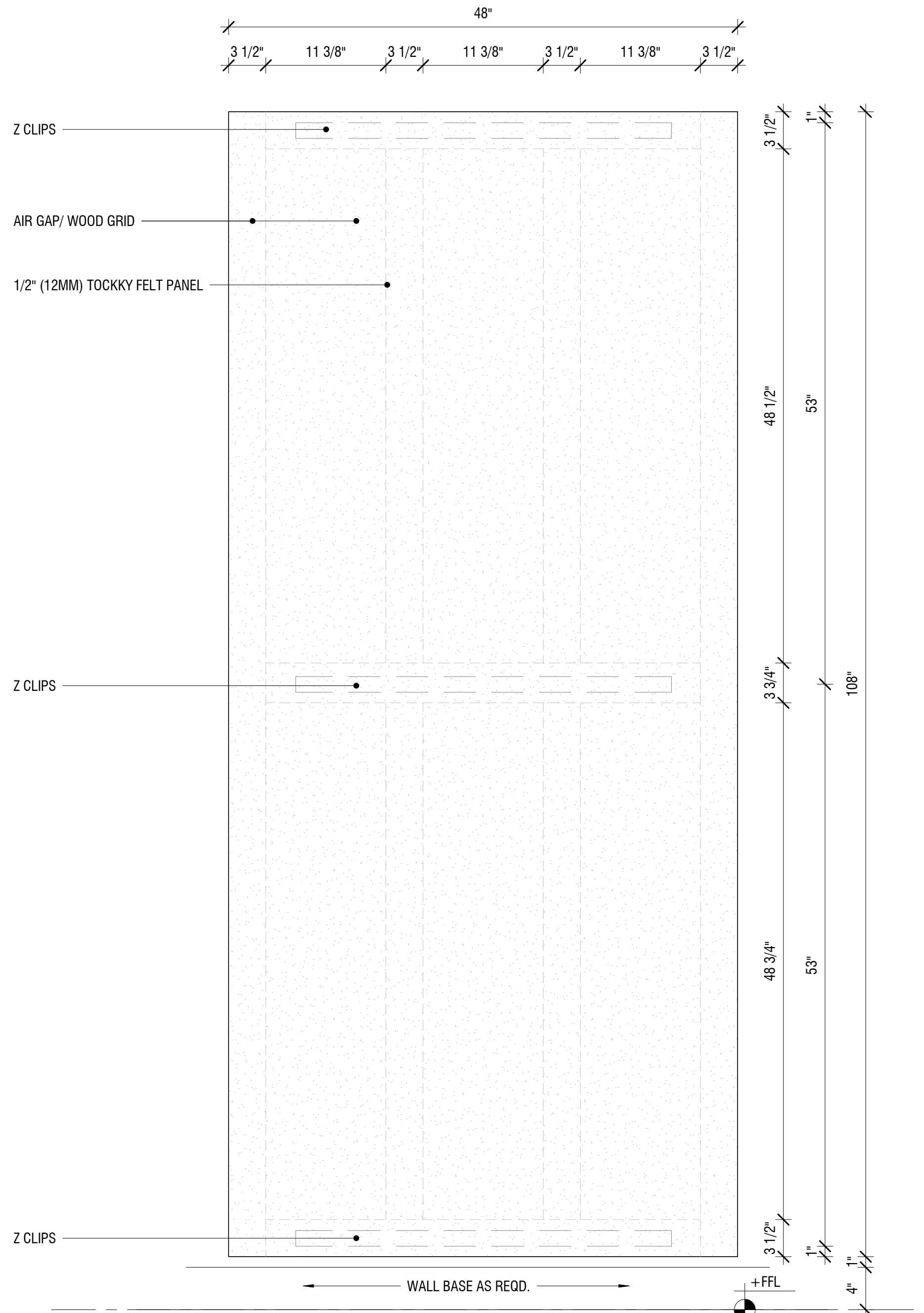
1/2" TOCKKY PANEL OMEGA DUAL PANEL W/BUILT-IN AIR GAP - 4'x9' - 1ST STYLE - ELEVATION 1 1/2" = 1'-0"
