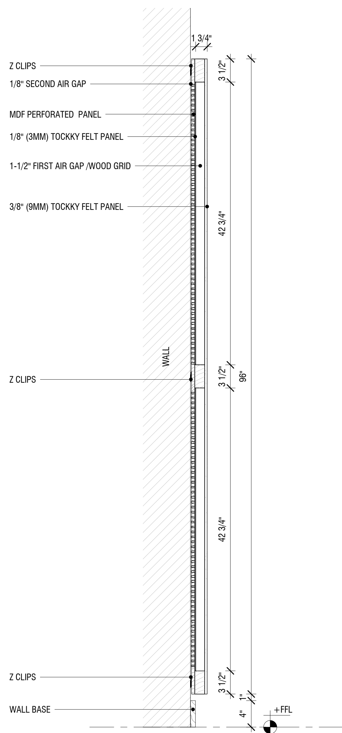
3/8" TOCKKY PANEL OMEGA DUAL PANEL W/BUILT-IN AIR GAP - 4'x8' - 1ST STYLE - TYP. SECTION 1 1/2" = 1'-0"
