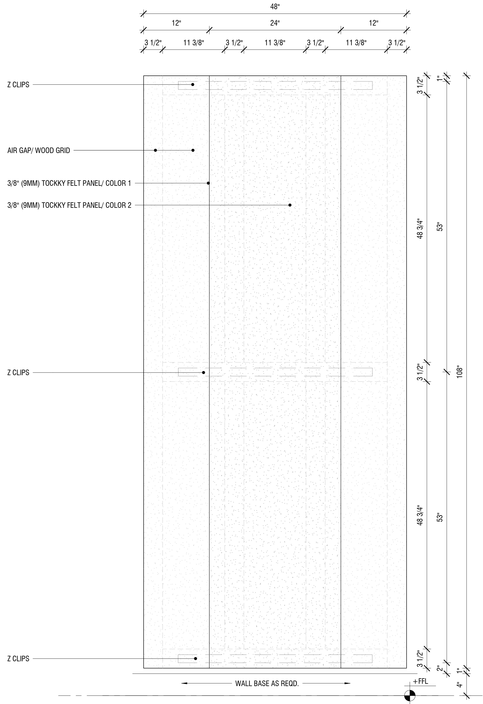
3/8" TOCKKY PANEL OMEGA DUAL PANEL W/BUILT-IN AIR GAP - 4'x9' - 2ND STYLE - ELEVATION 1 1/2" = 1'-0"
