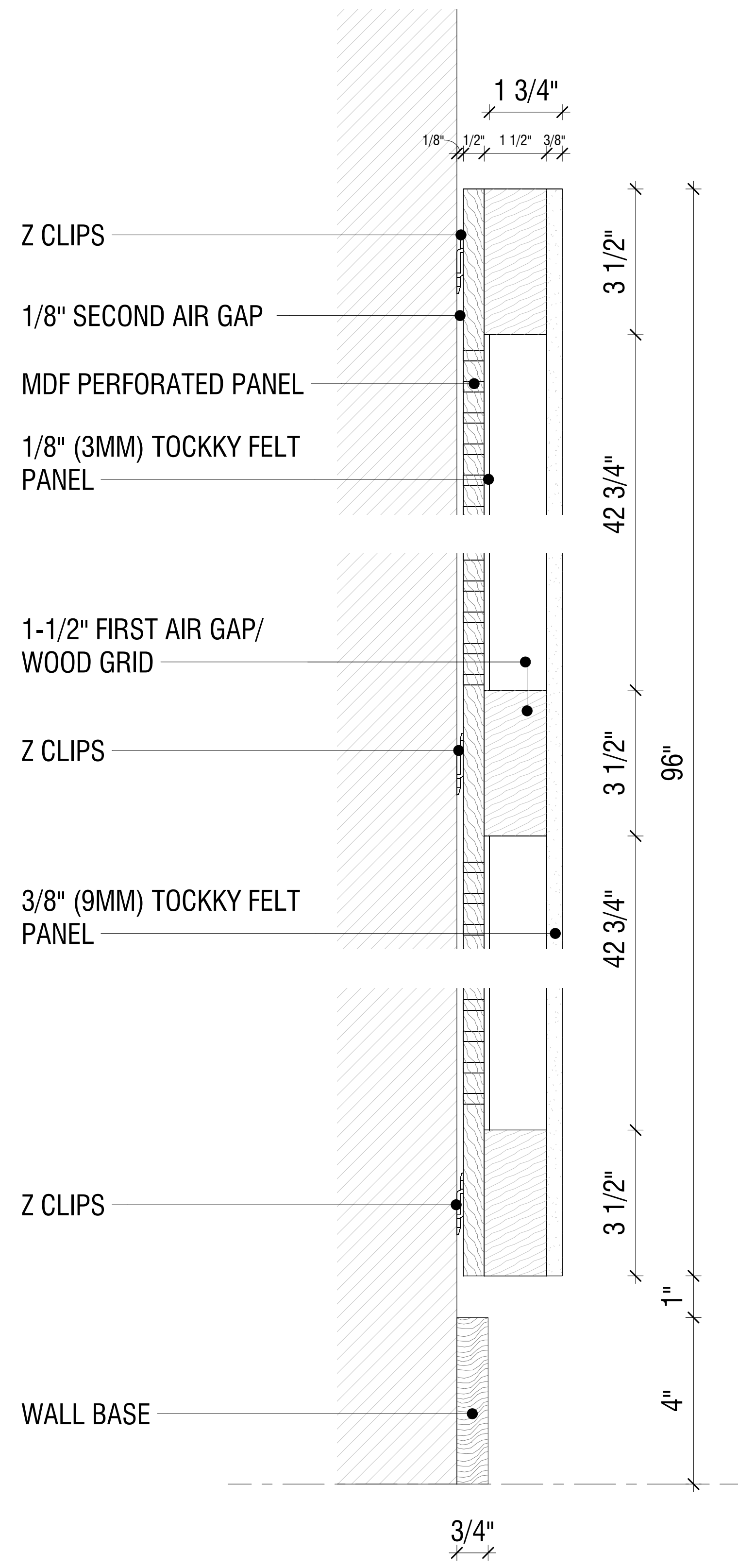
3/8" TOCKKY PANEL OMEGA DUAL PANEL W/BUILT-IN AIR GAP - 4'x8' - 1ST STYLE - SECTIONAL DETAIL 6" = 1'-0"
