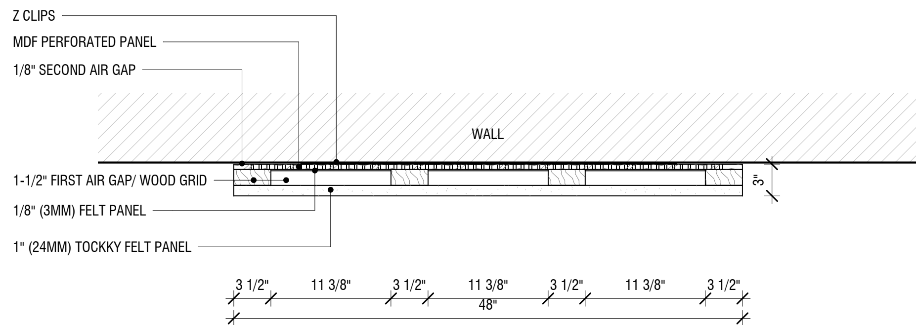
1" TOCKKY PANEL OMEGA DUAL PANEL W/BUILT-IN AIR GAP - 4'x9' - 1ST STYLE - PLAN VIEW 1 1/2" = 1'-0"
