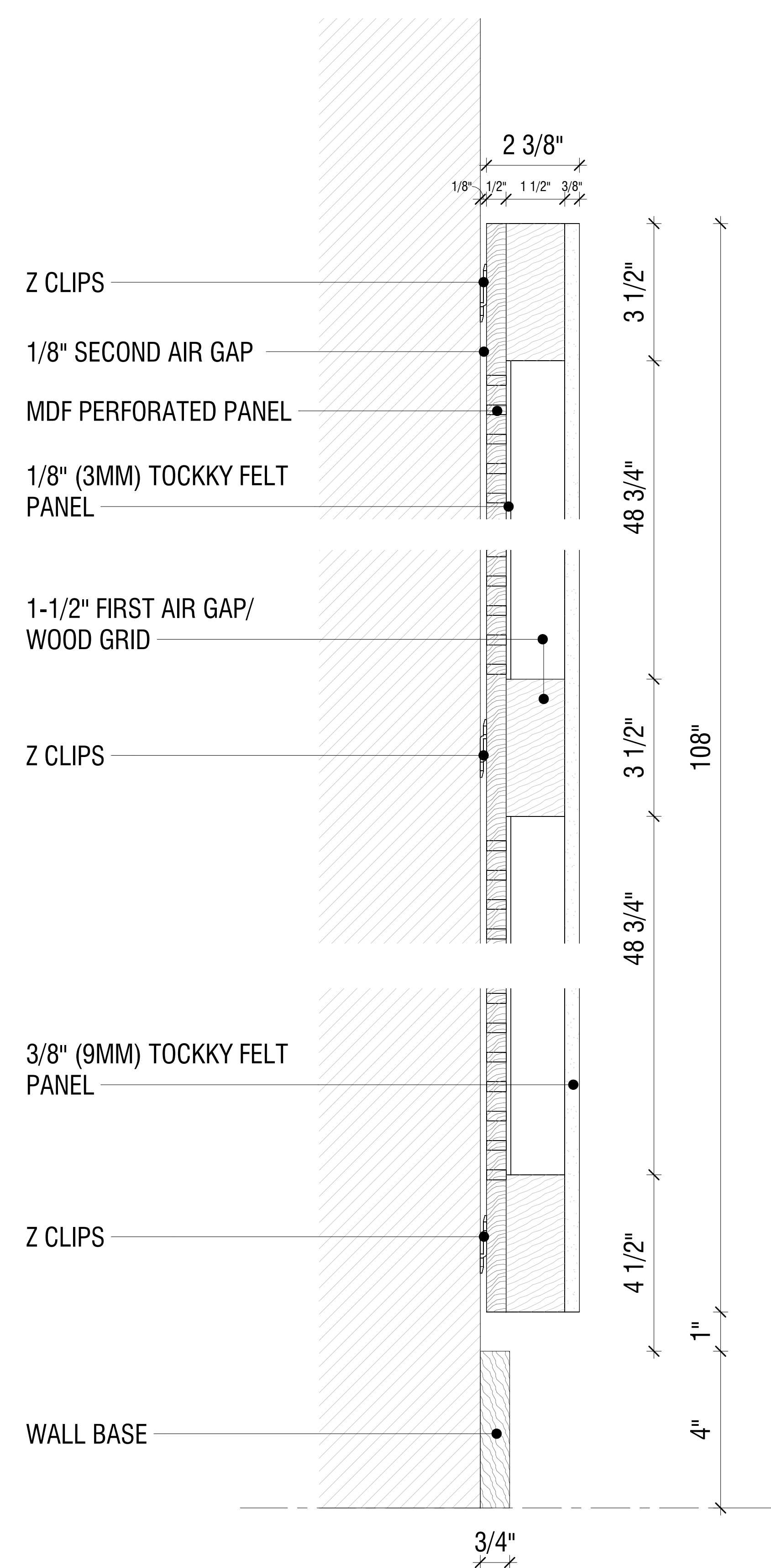
3/8" TOCKKY PANEL OMEGA DUAL PANEL W/BUILT-IN AIR GAP - 4'x9' - 1ST STYLE - SECTIONAL DETAIL ④ 6" = 1'-0"
