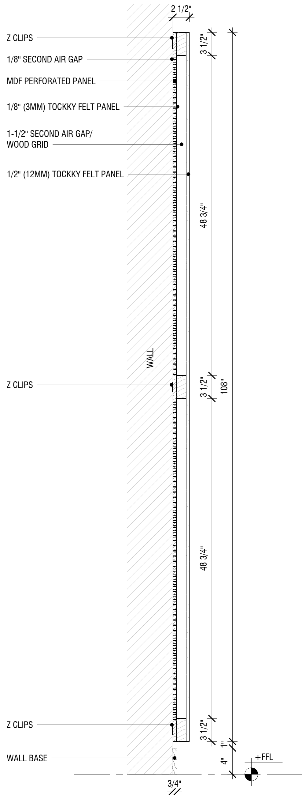
1/2" TOCKKY PANEL OMEGA DUAL PANEL W/BUILT-IN AIR GAP - 4'x9' - 1ST STYLE - TYP. SECTION 1 1/2" = 1'-0"
