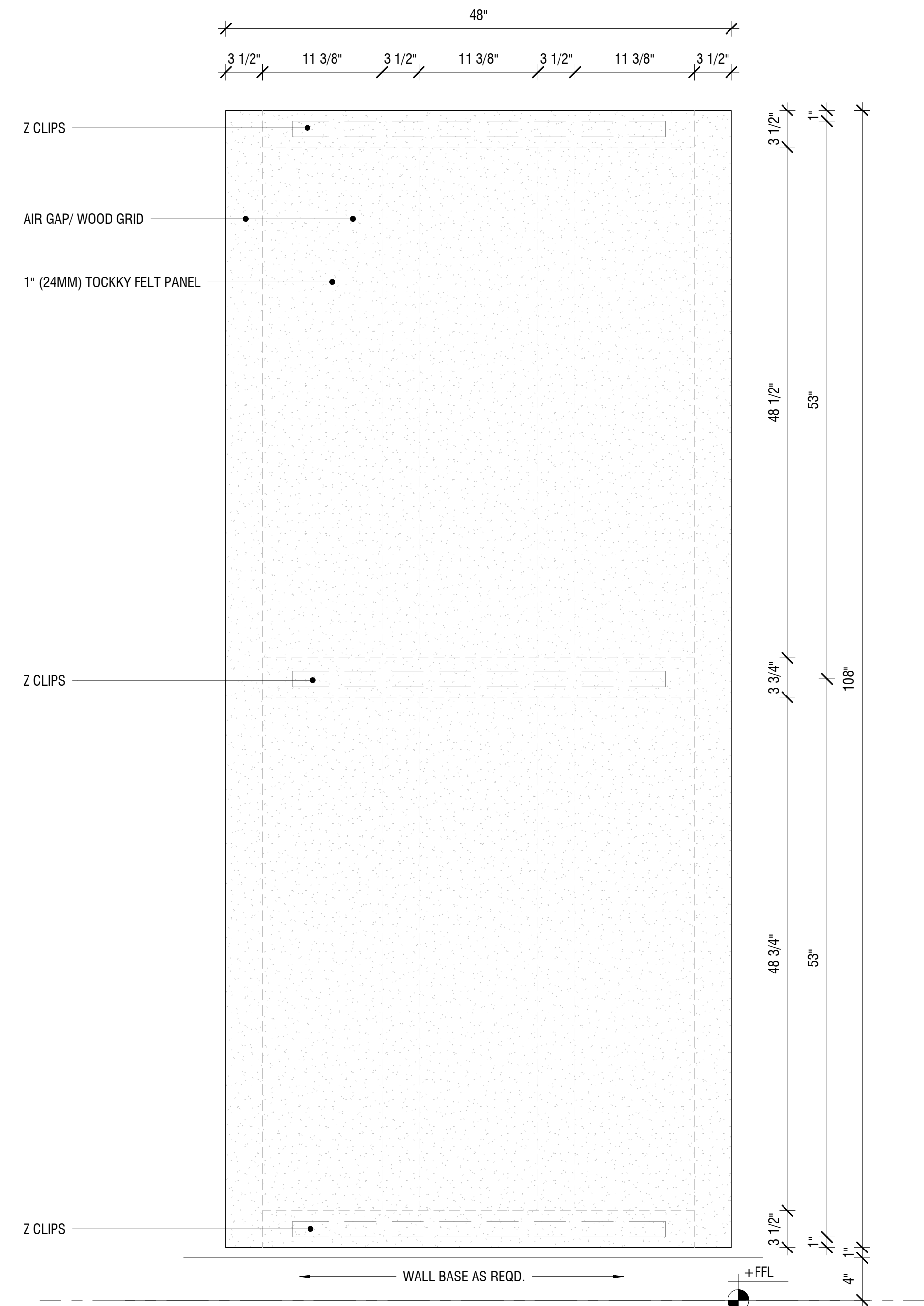
1" TOCKKY PANEL OMEGA DUAL PANEL W/BUILT-IN AIR GAP - 4'x9' - 1ST STYLE - ELEVATION 1 1/2" = 1'-0"
