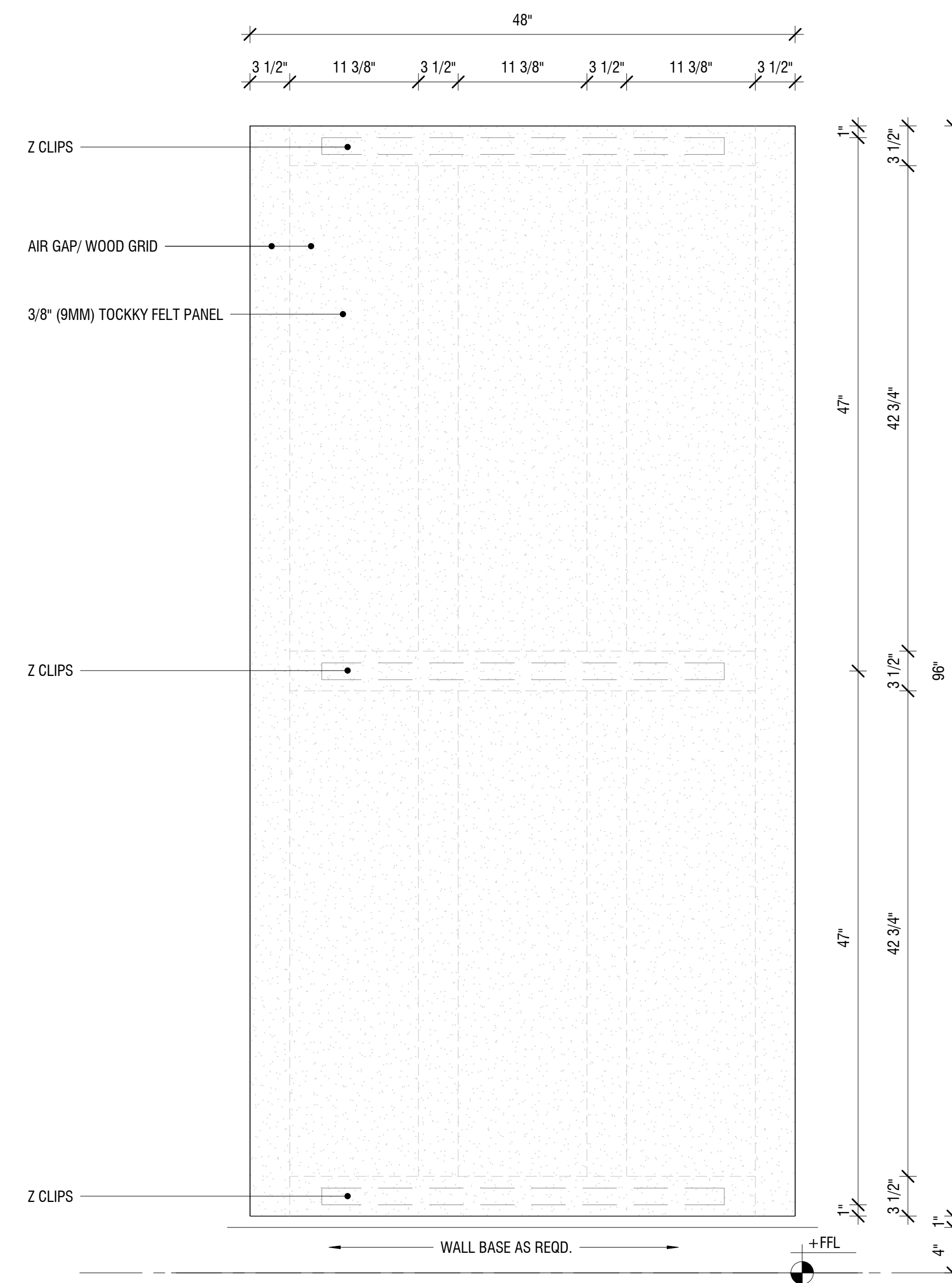
3/8" TOCKKY PANEL OMEGA DUAL PANEL W/BUILT-IN AIR GAP - 4'x8' - 1ST STYLE - ELEVATION 1 1/2" = 1'-0"
