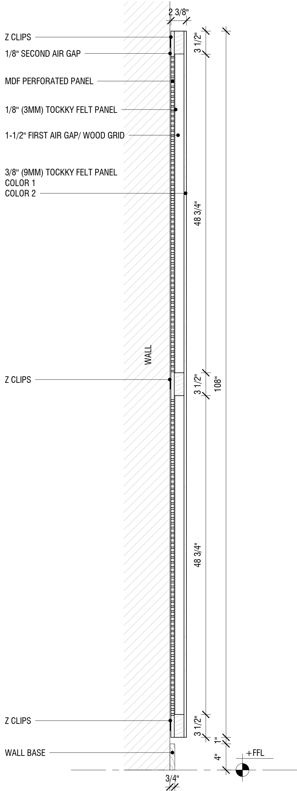
3/8" TOCKKY PANEL OMEGA DUAL PANEL W/BUILT-IN AIR GAP - 4'x9' - 2ND STYLE - TYP. SECTION 1 1/2" = 1'-0"
