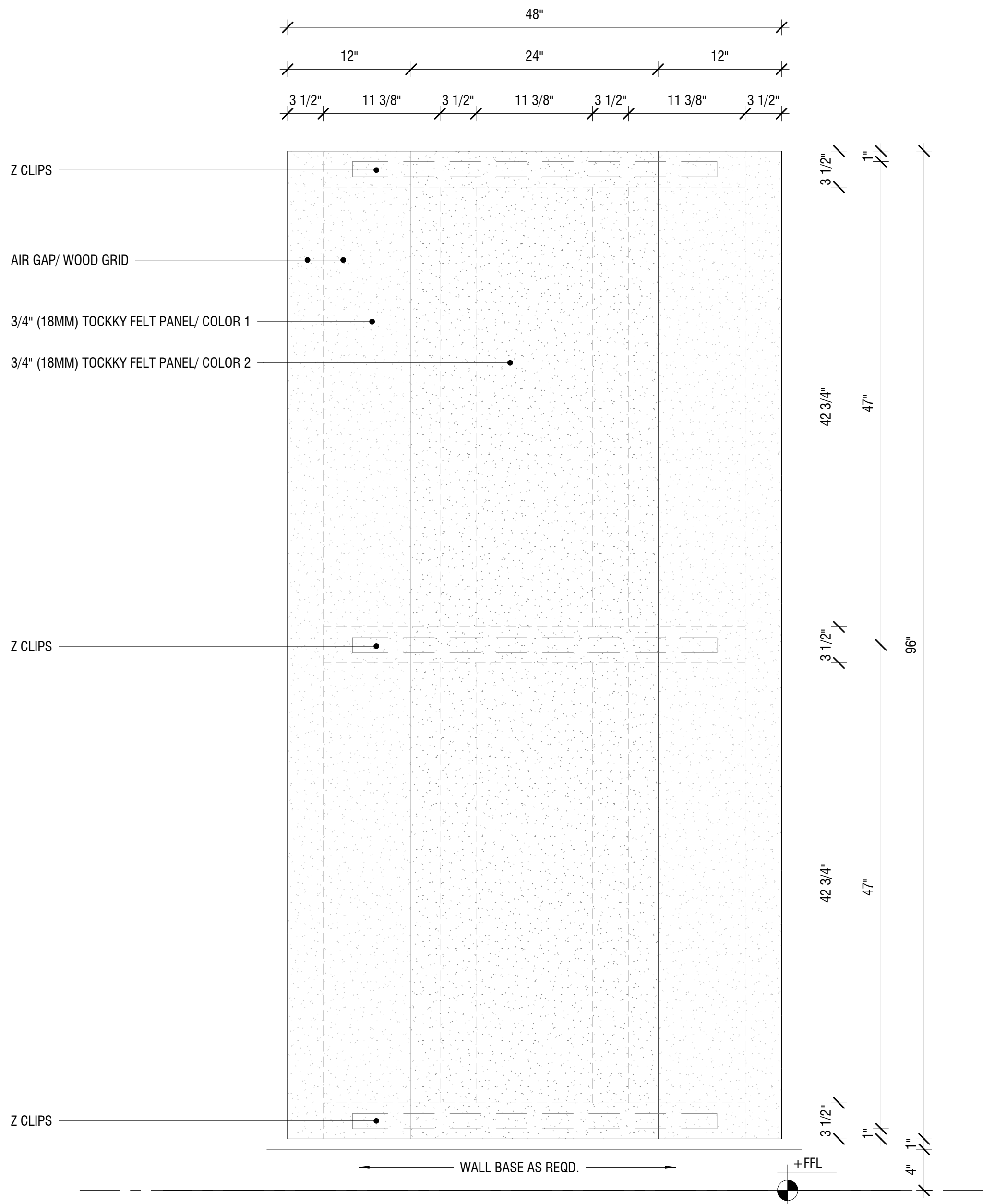
3/4" TOCKKY PANEL OMEGA DUAL PANEL W/BUILT-IN AIR GAP - 4'x8' - 2ND STYLE STYLE - ELEVATION ② 1 1/2" = 1'-0"
