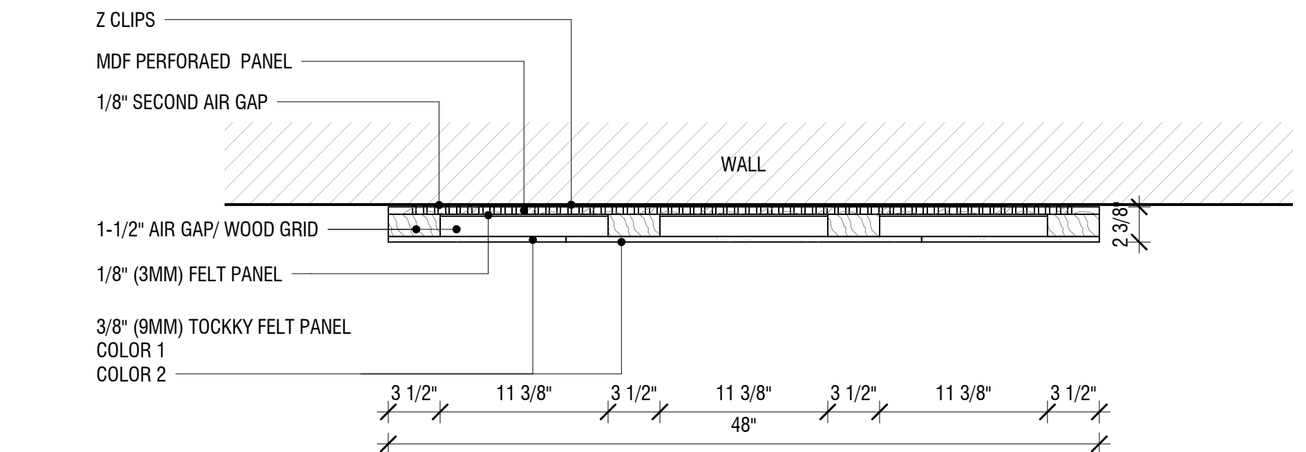
3/8" TOCKKY PANEL OMEGA DUAL PANEL W/BUILT-IN AIR GAP - 4'x9' - 2ND STYLE - PLAN VIEW 1 1/2" = 1'-0"
