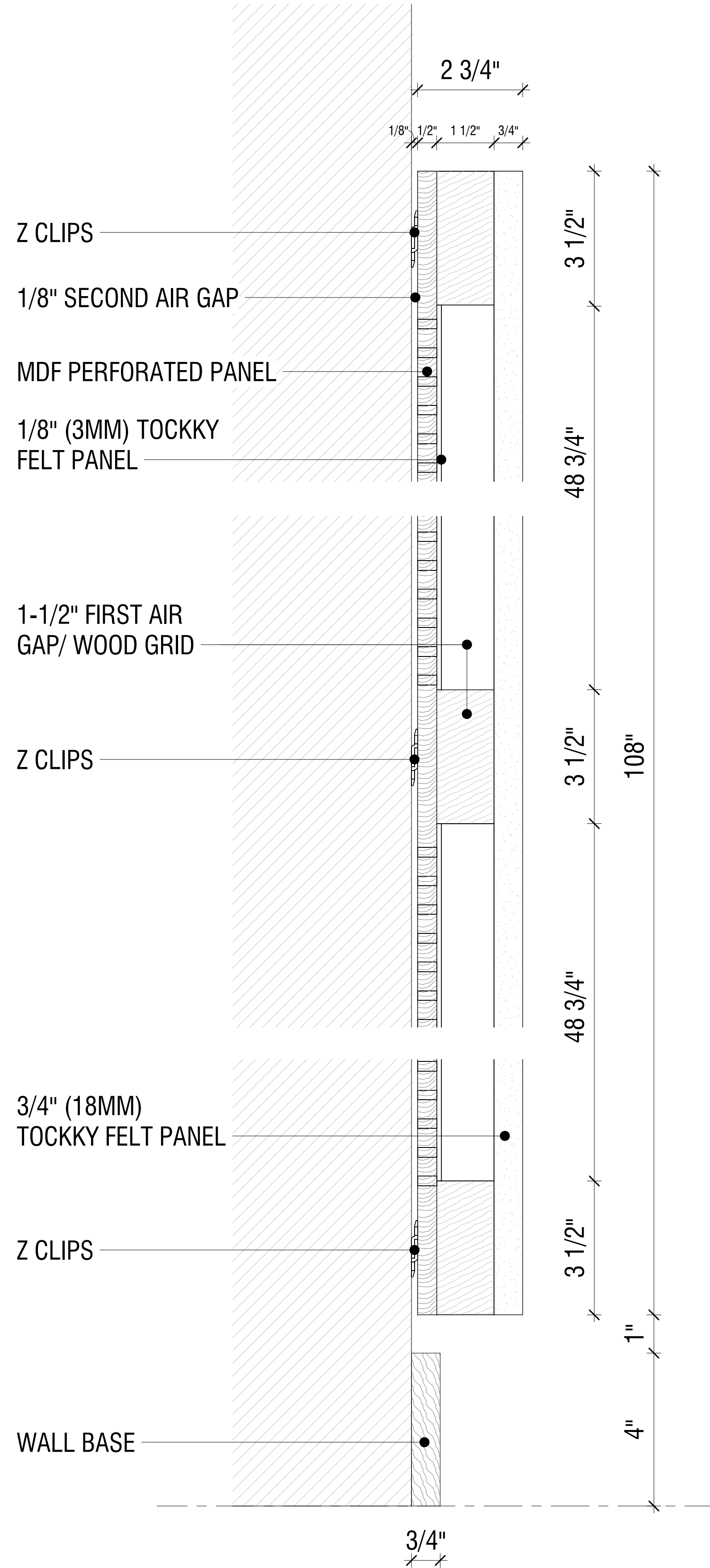
3/4" TOCKKY PANEL OMEGA DUAL PANEL W/BUILT-IN AIR GAP - 4'x9' - 1ST STYLE STYLE - SECTIONAL DETAIL 6" = 1'-0"
