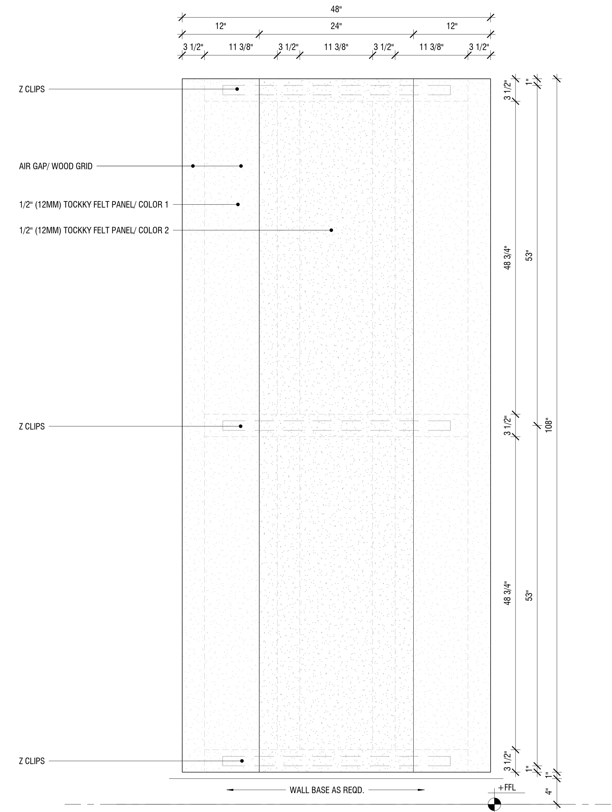
1/2" TOCKKY PANEL OMEGA DUAL PANEL W/BUILT-IN AIR GAP - 4'x9' - 2ND STYLE - ELEVATION 1 1/2" = 1'-0"
