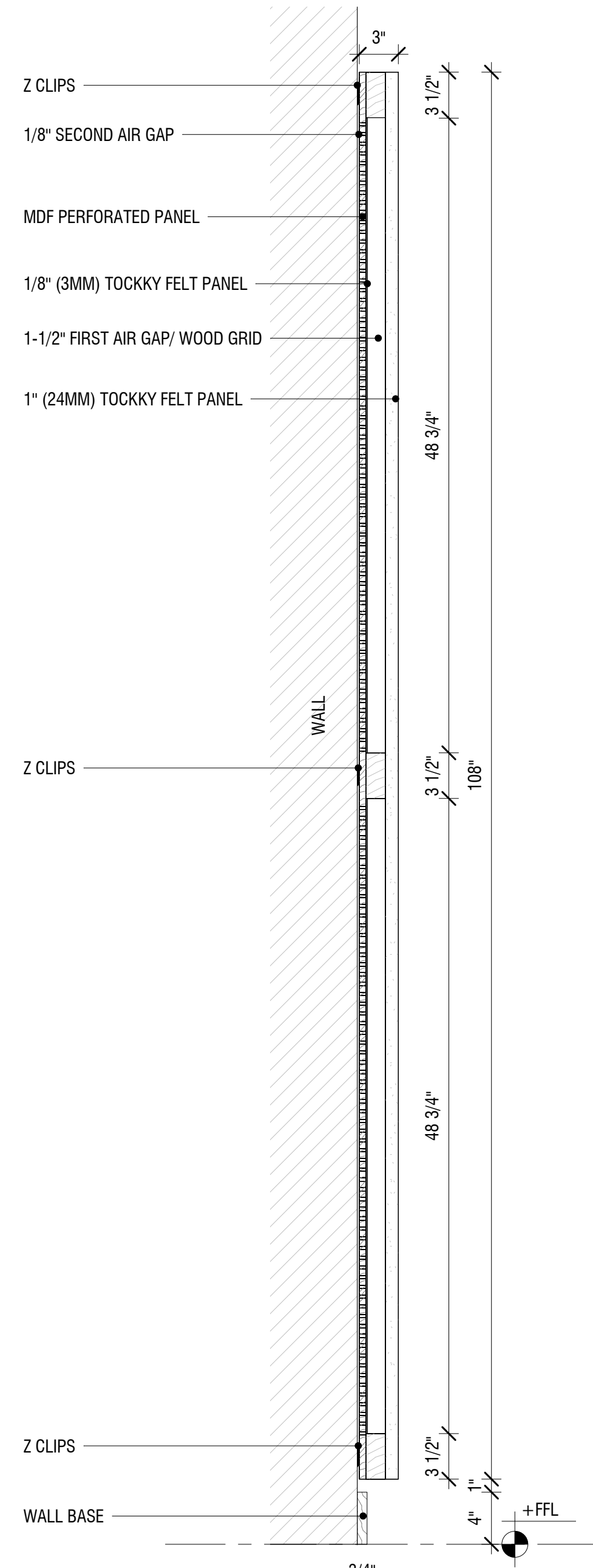
1" TOCKKY PANEL OMEGA DUAL PANEL W/BUILT-IN AIR GAP - 4'x9' - 1ST STYLE - TYP. SECTION 1 1/2" = 1'-0"
