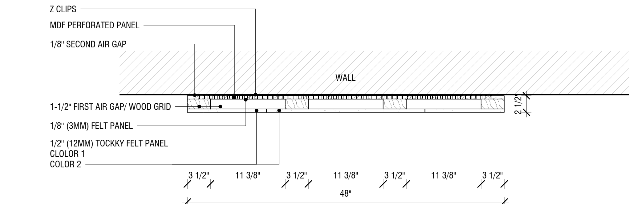
1/2" TOCKKY PANEL OMEGA DUAL PANEL W/BUILT-IN AIR GAP - 4'x9' - 2ND STYLE - PLAN VIEW 1 1/2" = 1'-0"
