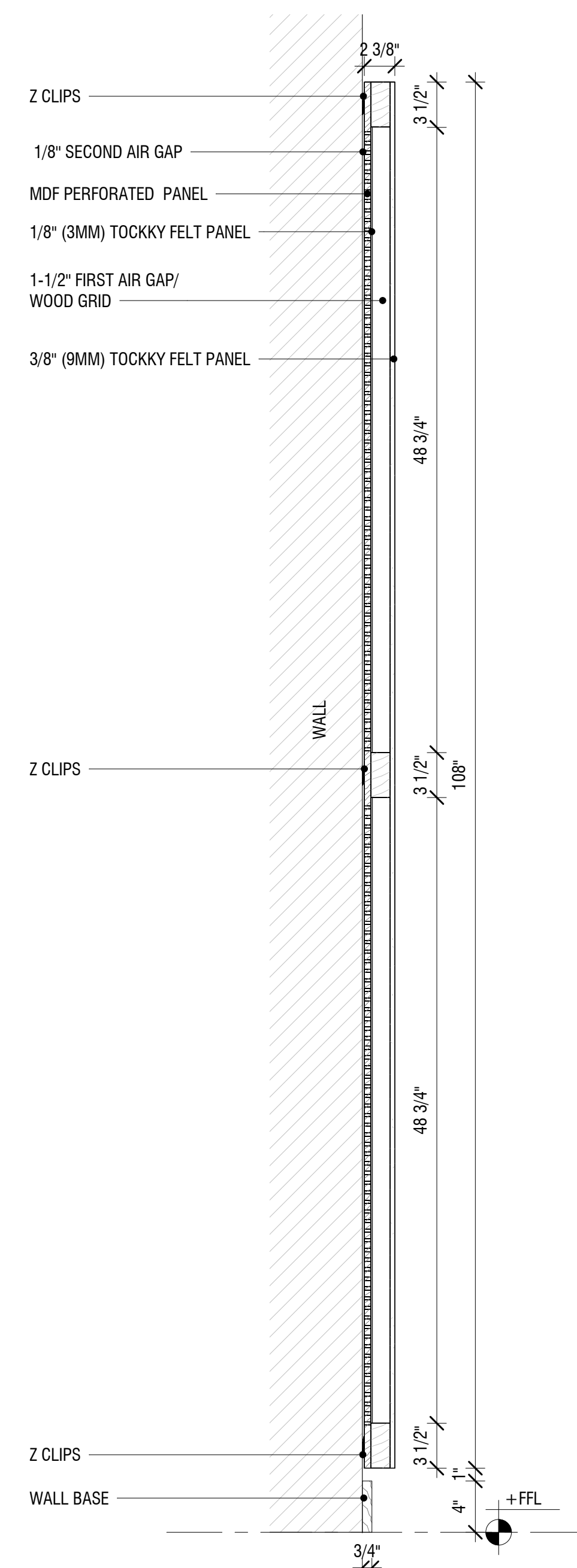
3/8" TOCKKY PANEL OMEGA DUAL PANEL W/BUILT-IN AIR GAP - 4'x9' - 1ST STYLE - TYP. SECTION ③ 1 1/2" = 1'-0"
