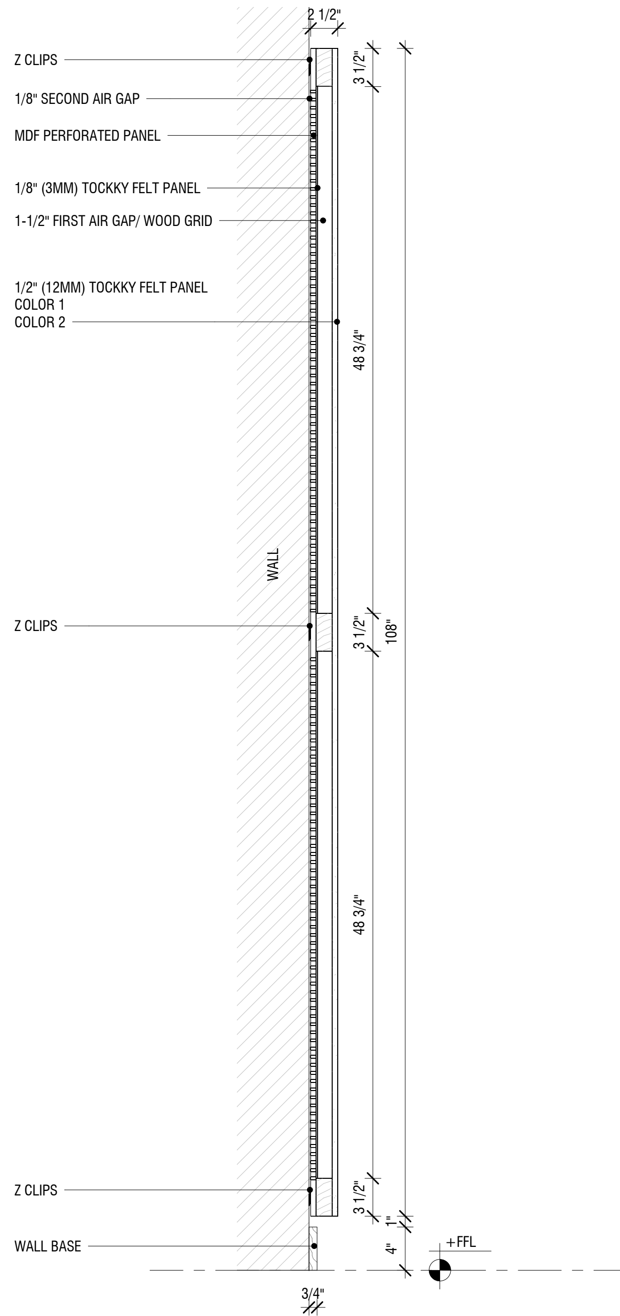
1/2" TOCKKY PANEL OMEGA DUAL PANEL W/BUILT-IN AIR GAP - 4'x9' - 2ND STYLE - TYP. SECTION 1 1/2" = 1'-0"
